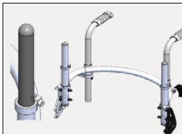
BRO4 Option with adjustable handles in the backrest frame. Crossbar curved, two radiuses.
